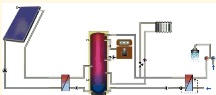
Figure 56: Hydraulic scheme of the solar-combi reference system for single and multi-family houses
