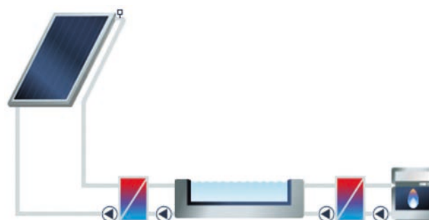
Figure 51: Hydraulic scheme of the swimming pool reference system
