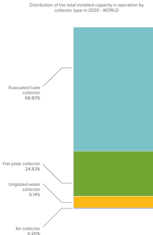
Figure 19: Distribution of the total installed capacity in operation by collector type in 2020 – WORLD
