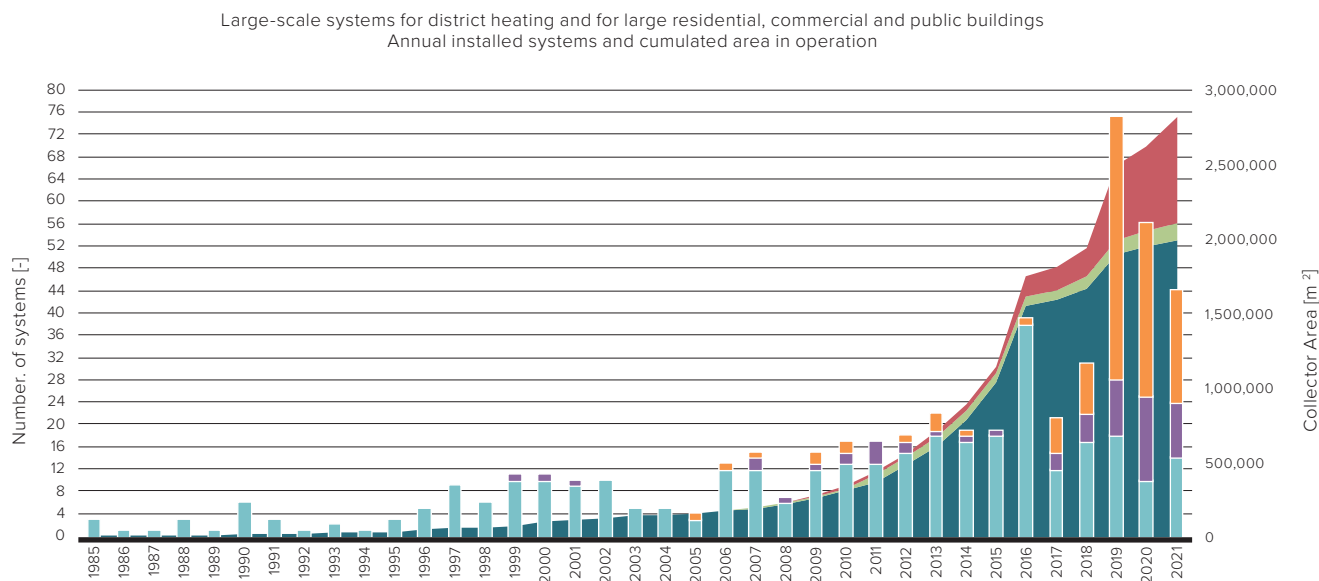
Figure 8: Large-scale systems for solar district heating and large residential, commercial and public buildings worldwide – annual achievements and cumulated area in operation in 2021
