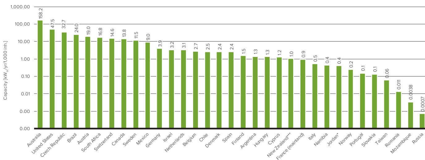
Figure 30: Total capacity of unglazed water collectors in operation in kW th per 1,000 inhabitants in 2020
