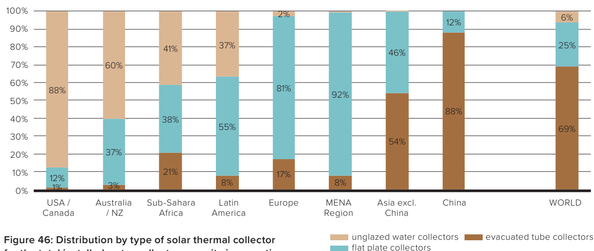
Distribution by type of solar thermal collector for the total installed water collector capacity in operation by the end of 2020
