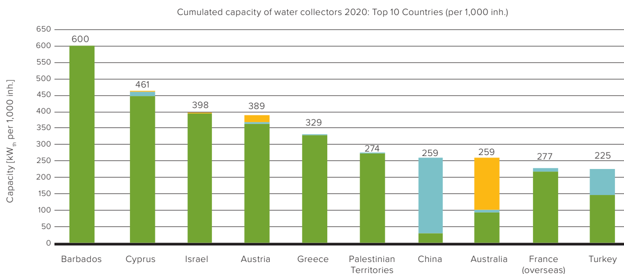
Figure 22: Top 10 countries of cumulated water collector installations per 1,000 inhabitants in 2020 (relative figures in kW th )
