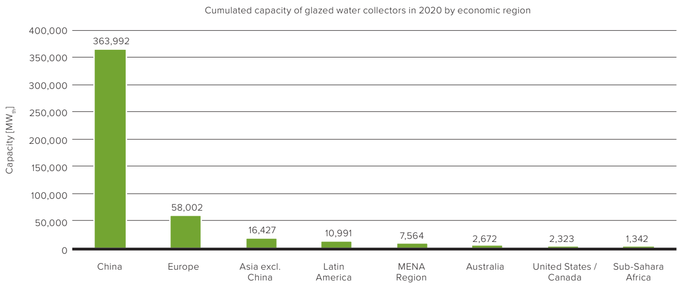
Figure 27: Total capacity of glazed flat plate and evacuated tube collectors in operation by economic region in 2020
