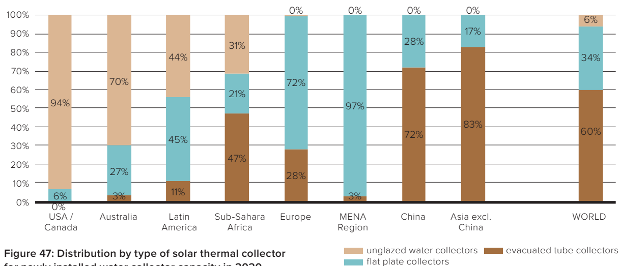
Distribution by type of solar thermal collector for newly installed water collector capacity in 2020
